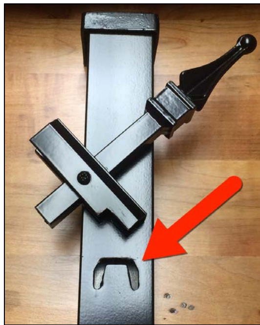
Figure 9 - The Fence Railing Will Insert Into the Routed Post Punch
