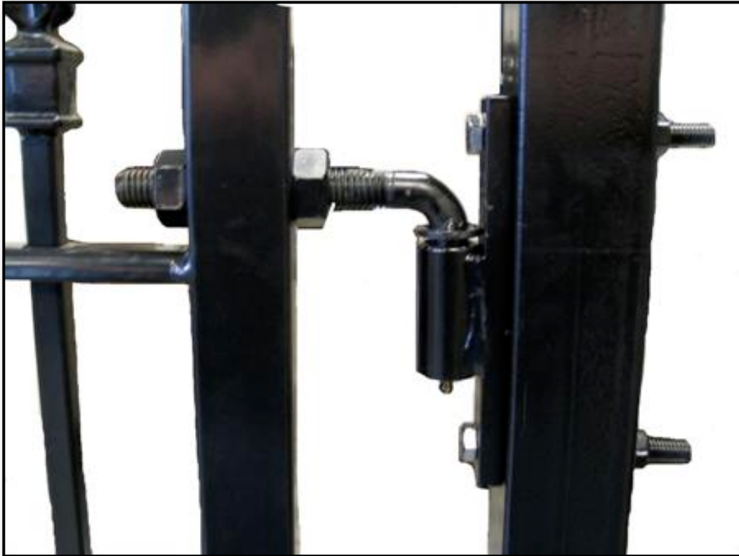
Figure 24 – An Installed J-Bolt Hinge. The Gate is on the Left and the Post is on the Right Side
