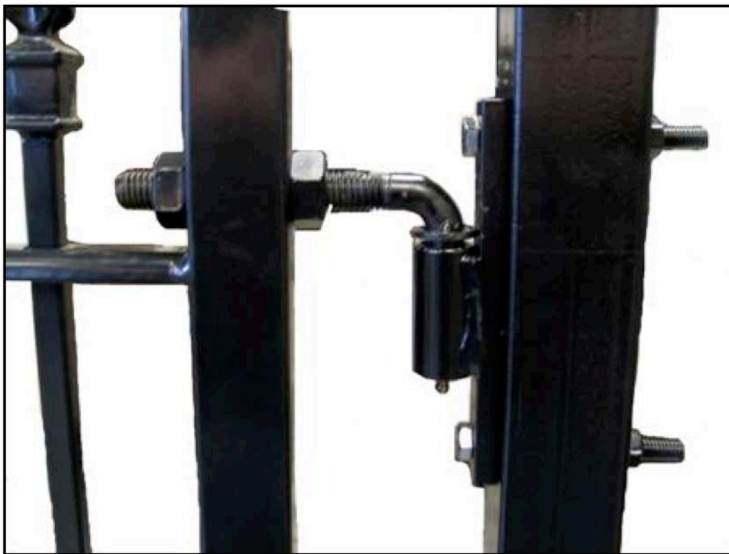
Figure 13 – An Installed J-Bolt Hinge. The Gate Frame is on the Left and the Post on the Right
