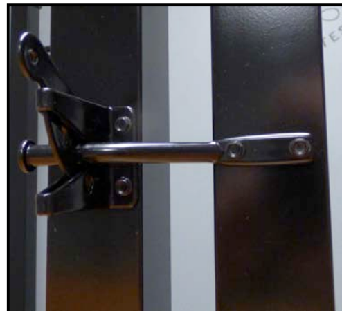
Figure 15 - Latch on Post (left) Arm on Gate (right)
