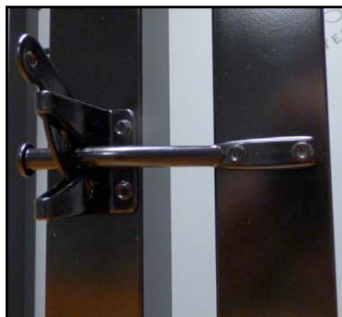
Figure 15 - Latch on Post (left) Arm on Gate (right)
